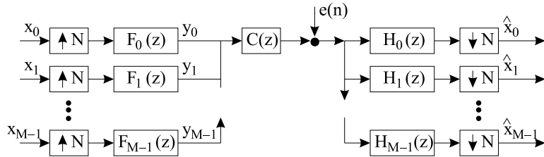
圖 1: An M -channel DMT system over a fading channel.
