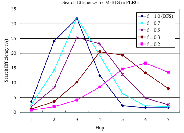
Fig. 6. Search Efficiency for M-BFS of various fraction parameters f in a power-law random graph with R = 1\%
