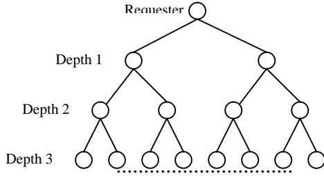
Fig. 1. A strictly binary tree with the requester at the root
