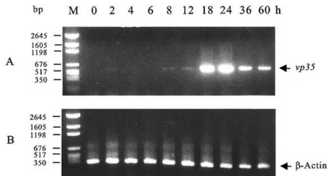
FIG. 6. Temporal transcription analysis of WSSV by RT-PCR. (A) RT-PCR with vp35 -specific primers. (B) Internal positive control: total RNA treated with DNase and amplified with actin-specific primers. The products were resolved in 1% agarose gel containing 0.5 µg/ml ethidium bromide. The size standards are indicated using pGEM DNA marker (Promega). Lane headings show hours pi.
