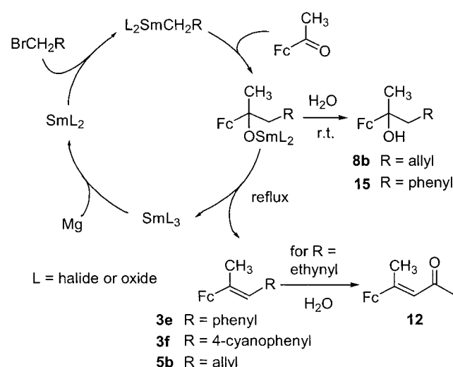
Figure 1. Proposed catalytic cycle for the reaction of acetylferrocene with halides in the presence of Mg and \text{SmI}_2 . The ligand L represents halide or oxide.
