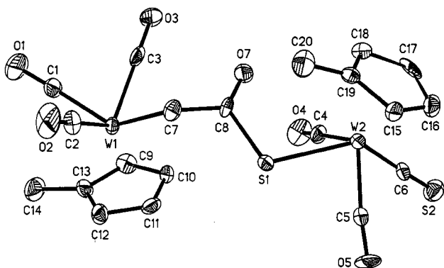
Fig. 2 An ORTEP drawing of W_2Cp'_2(CO)_5(CS)(\mu-CH_2COS) 5' .
