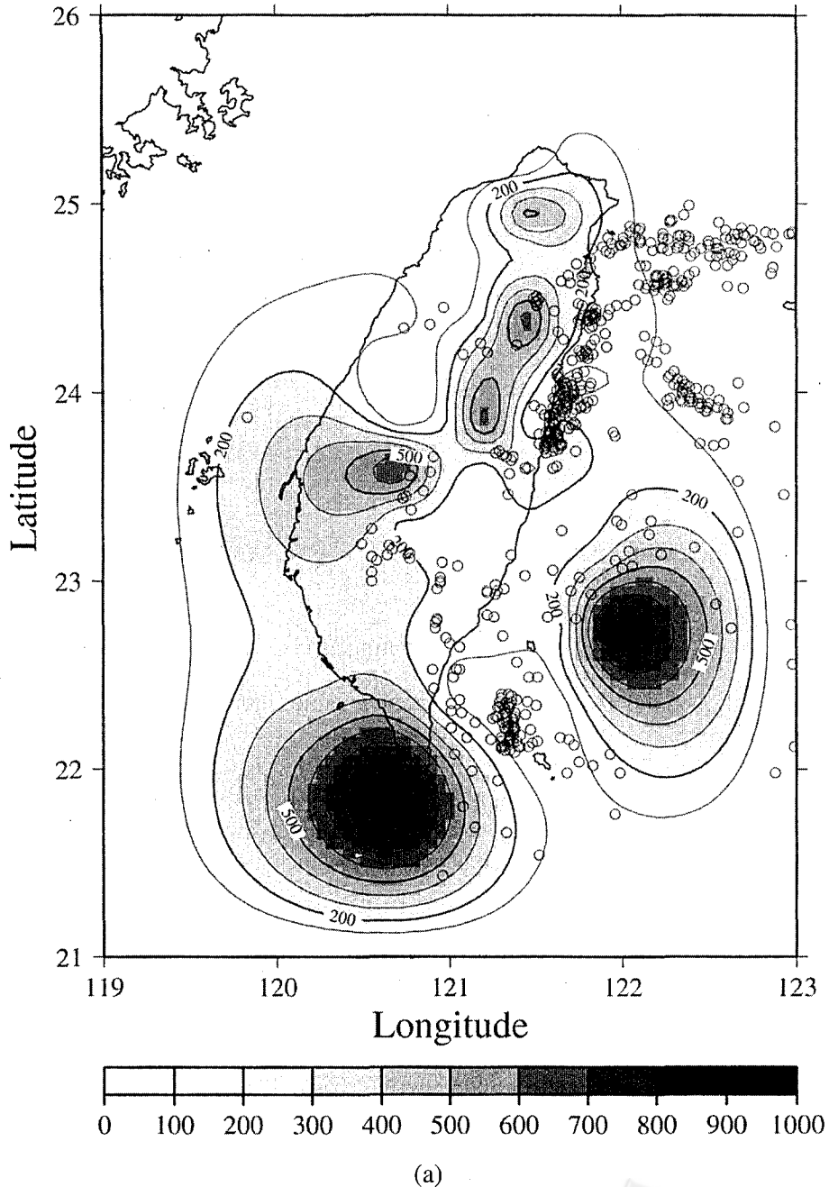
Fig. 5. Distribution of the Q_p values for each layer. These values are attributed to the center of each block, so that contour lines can be drawn. Contour lines are not drawn on zones through which no rays pass. Earthquakes located in the same block are shown with hollow circle symbols. The parameters of these earthquakes are mentioned in text.
