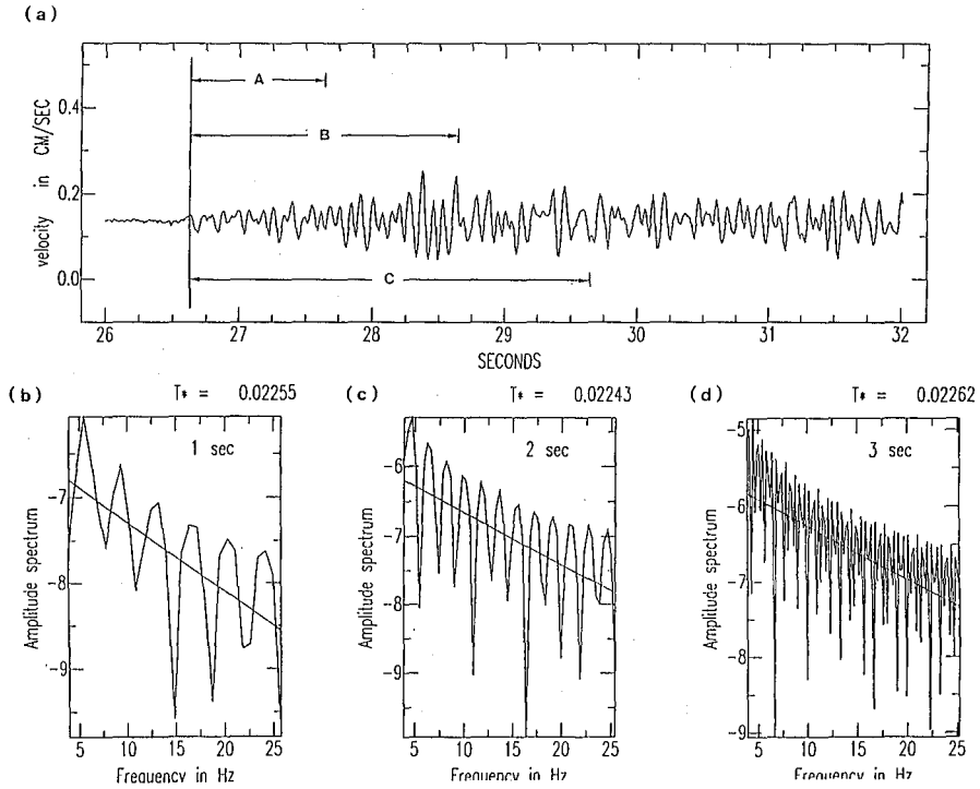
Fig. 3. (a) Seismogram used for calculating the t^* value and the three different time windows (denoted by A, B, and C); (b), (c) and (d) are the spectra calculated from the data truncated by time windows A, B, and C, respectively. The regression line and the t^* value are also shown in each diagram.
