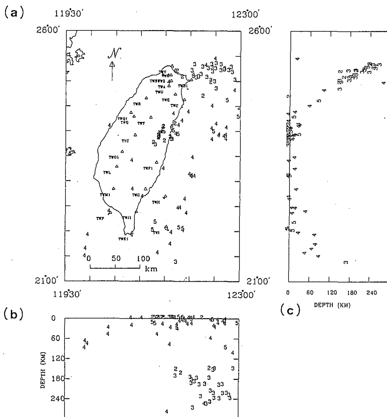
Fig. 2. Earthquakes and stations used in this study.
