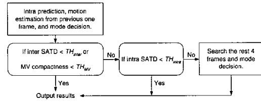
Fig. 3. Fast algorithm for multiple reference frames ME.
