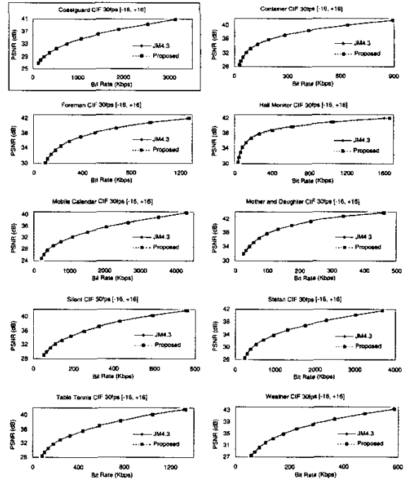
Fig. 5. Rate distortion curves of various sequences.
