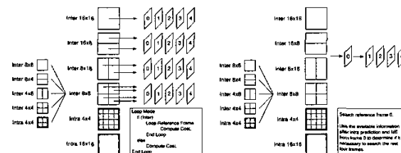
Fig. 1. Searching steps of intra/inter prediction with multiple reference frames in H.264 reference software and our method.
