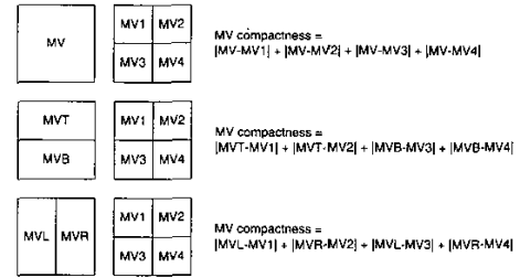
Fig. 2. Definition of MV compactness of a MB.
