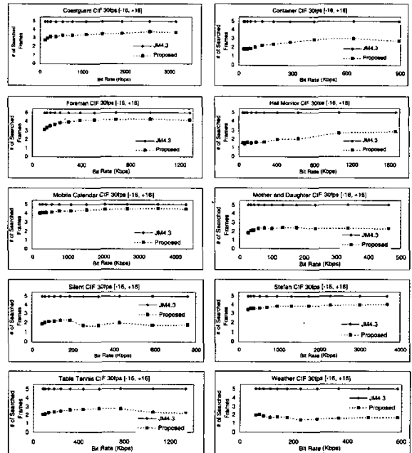
Fig. 6. Average searched frames for various sequences.
