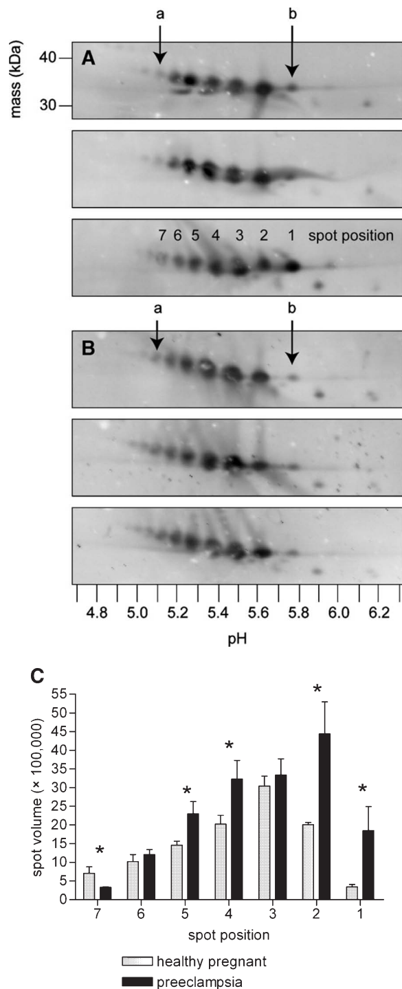
Fig. 3. Specific detection and quantitation of apolipoprotein E (apoE) isoforms in serum using 2-D Western blot analysis. 2-D Western blot analysis of 200 µg depleted serum from three women with preeclampsia (A) and three healthy pregnant women (B). Acidic (arrow a) and basic (arrow b) apoE isoforms, based on pI positions from serum 2DE, are indicated as shown. The volumes of individual spots 1–7 are shown as the mean \pm SEM of values derived from all six blots (C). Asterisks indicate significant differences between groups (all P < 0.05 ).
