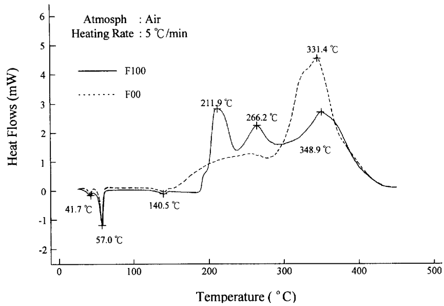
Fig. 5. DSC histograms of F00 and F100 feedstocks.
