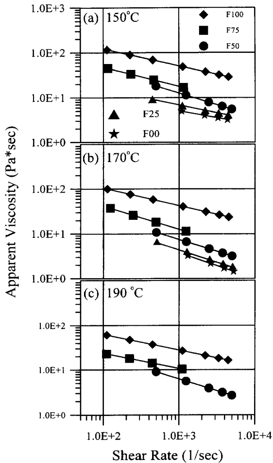
Fig. 2. Apparent viscosity of five feedstocks tested at temperatures either at 150, 170 or 190°C.
