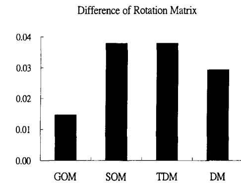
Fig. 2. Ensemble time-averaged differences of the origin vector and rotation matrix of the thigh coordinate system for the four methods.
