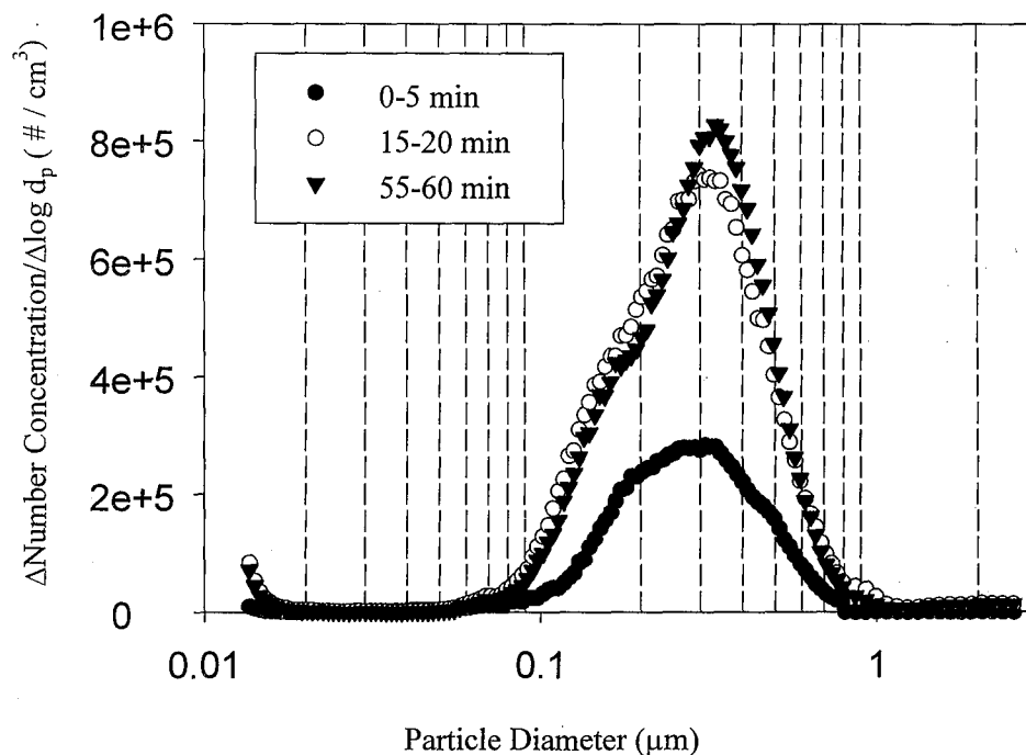
Figure 2 Size distributions of particles in black lignaloes smoke in the experimental chamber at various combustion times. Data in the range of 0.013- 0.80 \mu\text{m} were SMPS measurements and data in the range of 0.80-2.5 \mu\text{m} were APS measurements.
