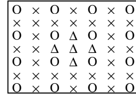
Figure 1. The input and output pixels in a window with size 7 \times 7 for SAMI scheme. The sample locations denoted O, X, and \Delta are the input, unknown, and output signals, respectively.
