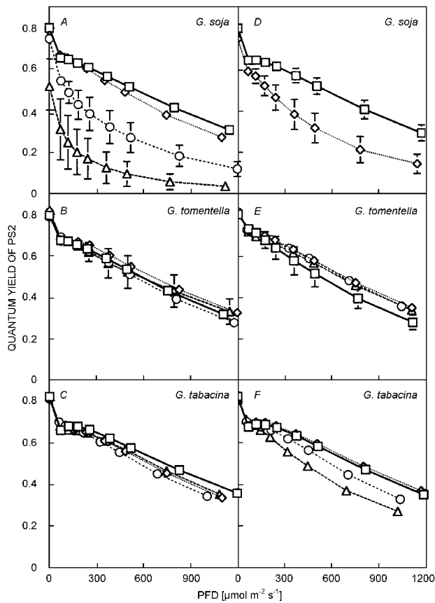
Fig. 2. The photon response curve of quantum yield of photosystem 2 of three wild soybean species ( G. soja , G. tomentella , and G. tabacina ), after one (A, B, C) and two (D, E, F) months of 0 (square), 17 (diamond), 51 (circle), and 85 (triangle) mM NaCl treatments. Vertical bars represent 1 S.E. of treatment ( n = 4 ).
