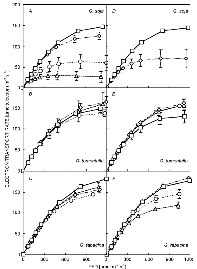
Fig. 3. The photon response curve of apparent electron transport rate of three wild soybean species ( G. soja , G. tomentella , and G. tabacina ) after one (A, B, C), and two (D, E, F) months of 0 (square), 17 (diamond), 51 (circle), and 85 (triangle) mM NaCl treatments. Vertical bars represent 1 S.E. of treatment ( n = 4 ).
