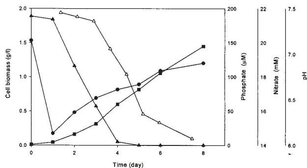
Figure 2. Cell growth and nutrient profile of Chlorella sp. NTU-H15 aerated with 15% CO 2 . ■, cell mass; ●, pH; ▲, phosphate; △, nitrate.
