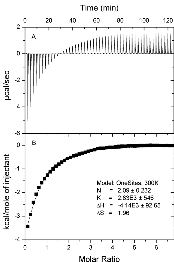
Figure 3. Isothermal titration calorimetry of the complex formation of ASTX (0.25 mM) and calcium ions (7.5 mM) at 300 K. (A) Raw data obtained from 48 automatic injections (6 \mu\text{L} each) of \text{Ca}^{2+} and (B) the integrated fitting curve showing the experimental points with the value of the parameter, n = 2 , by using a one-site binding fitting function.
