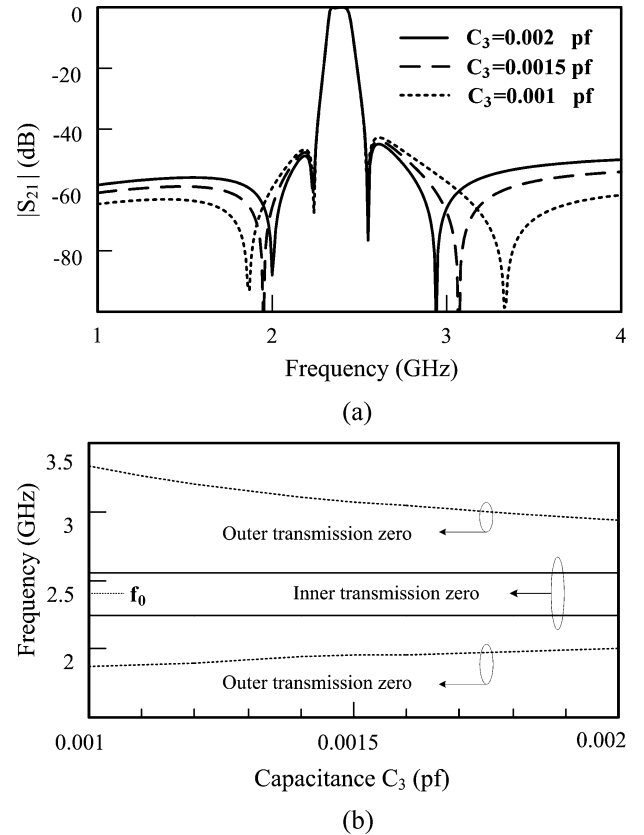
Fig. 8. (a) Simulated responses of the filter circuit model [see Fig. 6(b)] for various values of C_3 . (b) Curves to relate the transmission-zero frequencies to the values of C_3 ( f_0 = 2.4 GHz, Z_1 = 50 \Omega , \theta_1 = 75.4^\circ , \theta'_1 = 86.9^\circ , L = 0.11 nH, C_1 = 0.316 pF, C'_1 = 0.0279 pF, C_2 = 0.0125 pF).
