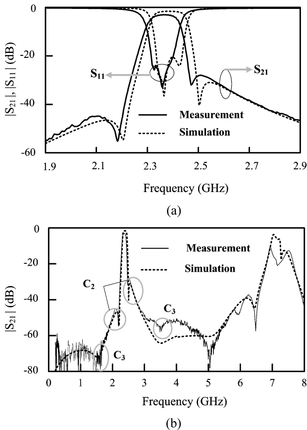
Fig. 10. Measured and simulated results of the proposed fourth-order microstrip filter in Fig. 6(a). (a) Narrow- and (b) wide-band frequency responses ( l_3 = 17.3 mm, l_4 = 27.3 mm, d_1 = 0 mm).
