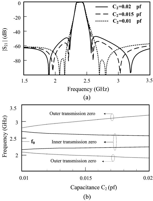
Fig. 7. (a) Simulated responses of the filter circuit model [see Fig. 6(b)] for various values of C_2 . (b) Curves to relate the transmission-zero frequencies to the values of C_2 ( f_0 = 2.4 GHz, Z_1 = 50 \Omega , \theta_1 = 75.4^\circ , \theta'_1 = 86.9^\circ , L = 0.11 nH, C_1 = 0.316 pF, C'_1 = 0.0279 pF, C_3 = 0.001 pF).
