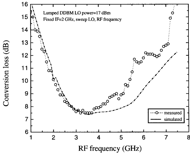
Fig. 2. Conversion loss of the DDBM, with a fixed IF frequency of a 2 GHz.
