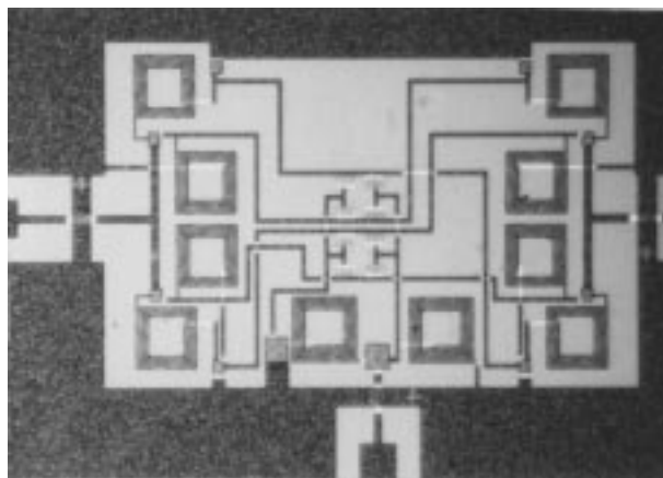
Fig. 1. (a) The circuit schematic diagram and (b) photograph of the lumped MMIC DDBM.
