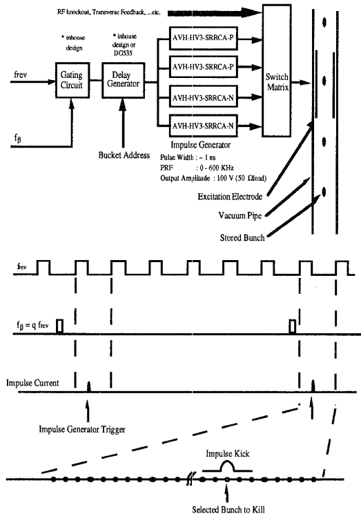
Figure 2. Nanosecond bunch killer
