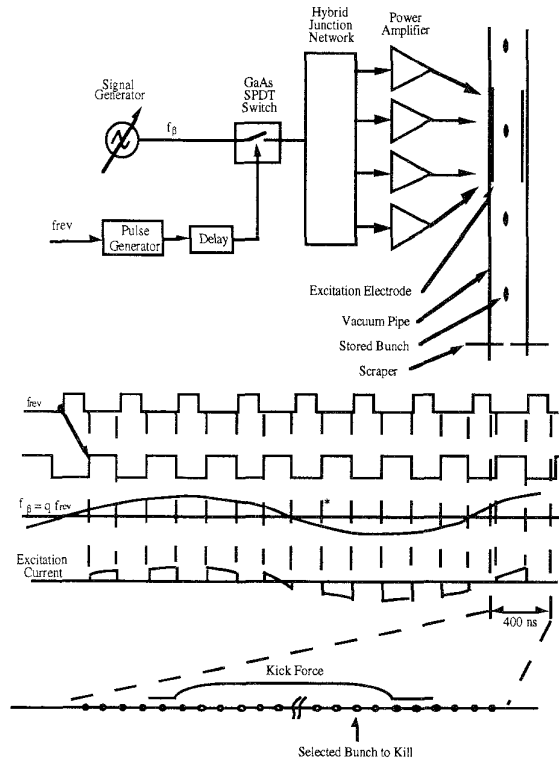
Figure 1. Multibunch filling pattern shaper
