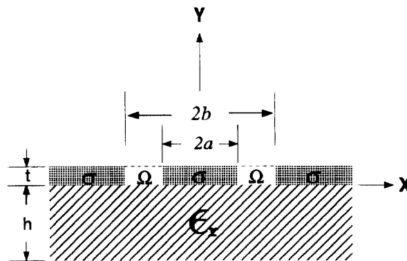
Fig. 1: Cross section of coplanar waveguide.
