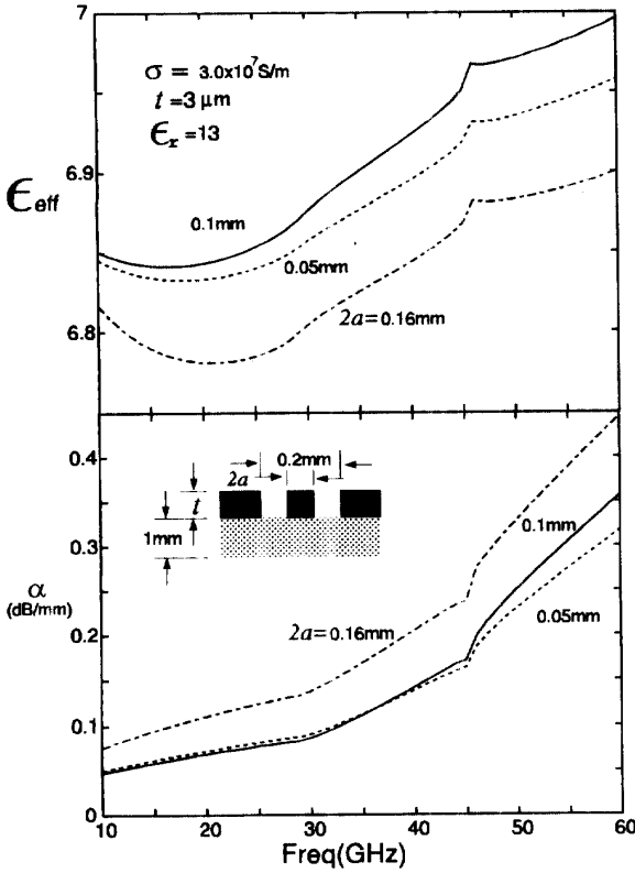
Fig. 4: Effective dielectric constant \epsilon_{eff} and attenuation constant \alpha versus frequency with strip width 2a as parameters.
