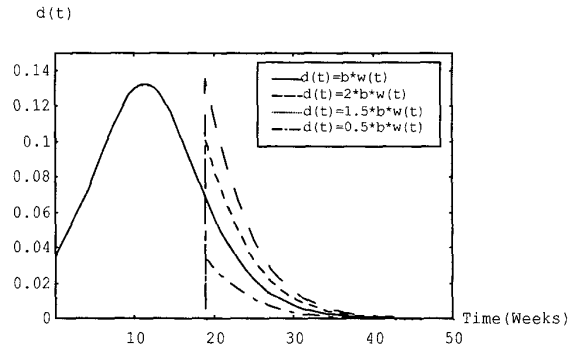
Figure 1: The detectability of faults during software testing and operational phase for Ohba's data set.
