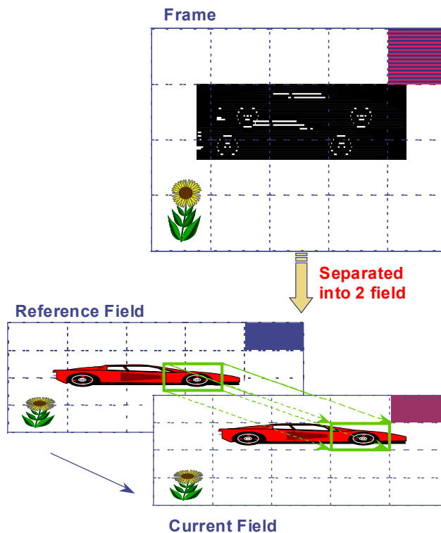
Fig. 4. Block matching by motion estimation method.
