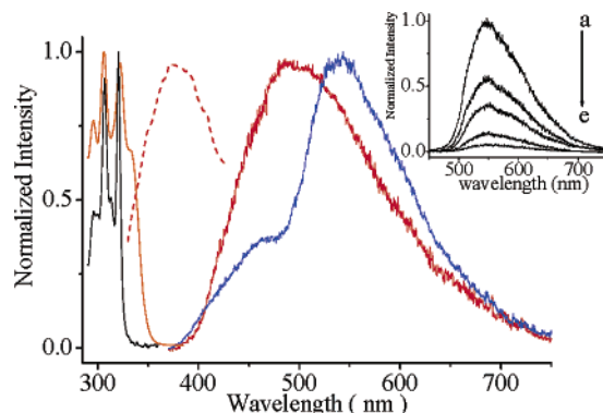
Figure 2. Absorption of L (black —) and 1 (orange —) at 298 K in THF; emission of 1 in a single crystal at 298 (red —) and 77 K (blue —); (red - - -) excitation spectrum of solid 1 at 298 K. Inset: spectral temporal evolution of solid 1 at 77 K acquired at a delay time of (a) 1, (b) 2, (c) 5, (d) 15, and (e) 30 \mu\text{s} .
