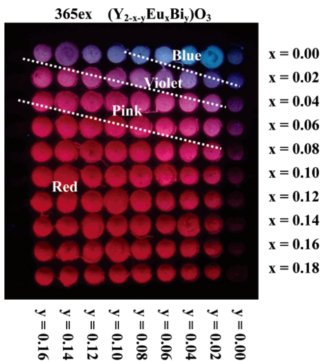
Figure 3. Composition map and photoluminescence photography of the library excited under 365 nm UV light for (Y_{2-x}Eu_xBi_{1-y})O_3 .
