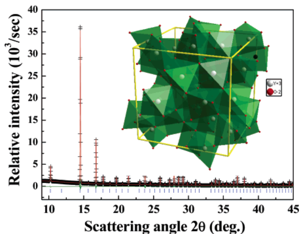
Figure 2. Observed (crosses), calculated (solid line), and differences (bottom) synchrotron XRD pattern of (Y_{2-x}Eu_xBi_{1-y})O_3 ( x = 0.16 , y = 0.16 ) at 300 K with \lambda = 0.7749 Å. Bragg reflections are indicated by tick marks. An ideal crystal structure is also shown in the inset.
