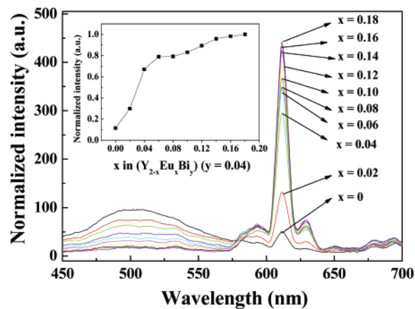
Figure 4. Emission spectrum of (Y_{2-x}Eu_xBi_{1-y})O_3 ( y = 0.04 ) with different Eu^{3+} contents. The normalized intensity as a function of x is also shown in the inset.
