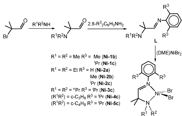
Scheme 1 Synthesis of ligands and nickel catalysts.
