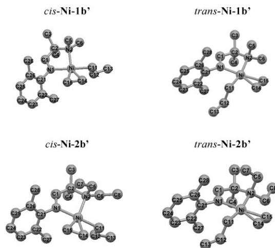
Fig. 2 Calculated structures for the geometrical isomers of (L-1b)Ni(C 2 H 4 )( n Pr) (Ni-1b') and (L-2b)Ni(C 2 H 4 )( n Pr) (Ni-2b').
