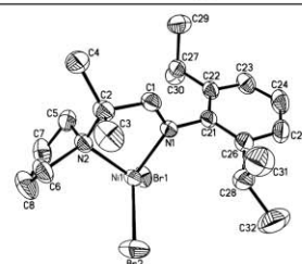
Fig. 1 ORTEP drawings of the nickel complexes. All hydrogen atoms are omitted for clarity. Ni-1b (the one that does not have disorder in the asymmetric unit is shown).
