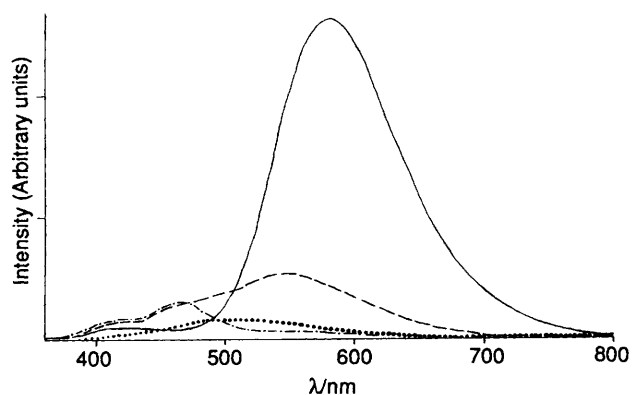
Fig. 3 Emission spectra of [\text{Au}_2\text{L}_3]^{2+} ( 1 \times 10^{-4} mol \text{dm}^{-3} ) in degassed acetonitrile ( \cdots ) and in the presence of \text{CF}_3\text{CO}_2\text{H} ( 1 \times 10^{-3} mol \text{dm}^{-3} , -\cdot-\cdot- ), \text{AgCF}_3\text{SO}_3 ( 1 \times 10^{-3} mol \text{dm}^{-3} , ---- ) or [\text{Cu}(\text{MeCN})_4]\text{PF}_6 ( 1 \times 10^{-3} mol \text{dm}^{-3} , --- )
