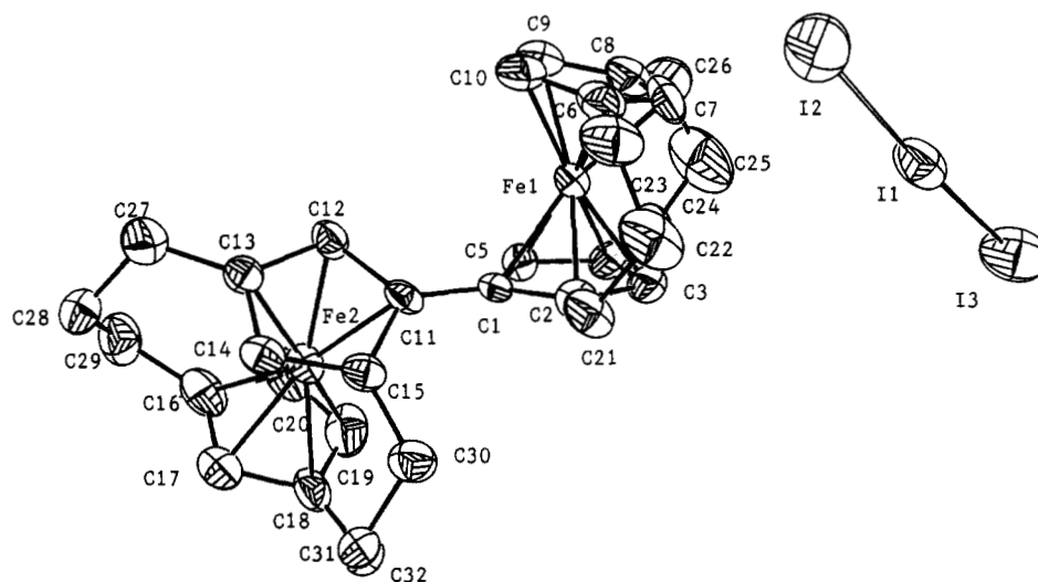
Figure 3. ORTEP drawing for 18a with 30% thermal ellipsoids.
