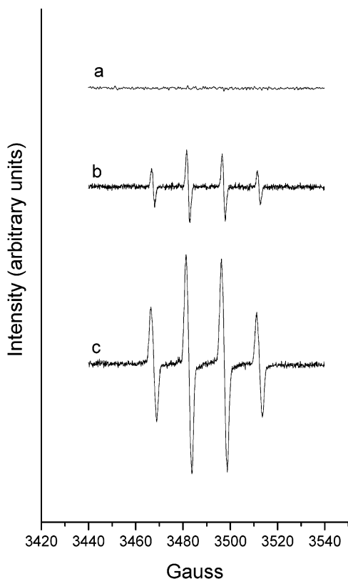
Figure 7. Spin trapping/EPR spectra of \cdot\text{DMPO-OH} radical intensity (liquid phase at room temperature) arising from different solids reacted with \text{H}_2\text{O}_2 : (a) V-MCM-41 after calcinations at 560 °C, zero intensity indicates all of the \text{V}^{4+} being converted to \text{V}^{5+} ; (b) MCM41-NH 2 -(VO)-H 2 O; and (c) silica gel-NH 2 -(VO)-H 2 O samples. We note that the intensity of \cdot\text{DMPO-OH} radicals is proportional to the amount of \text{V}^{4+} available for the oxidation reaction of \text{H}_2\text{O}_2 .
