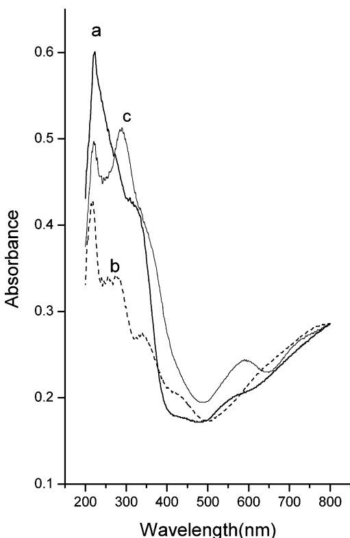
Figure 3. Diffuse reflectance UV-vis spectra of the following solids: (a) MCM41-NH 2 -(VO)-H 2 O (after heating in air at 100 °C for 24 h), (b) MCM41-NH 2 -(VO)-EtOH, and (c) MCM41-NH 2 -(VO)-EtOH (after heating in air at 100 °C for 24 h).
