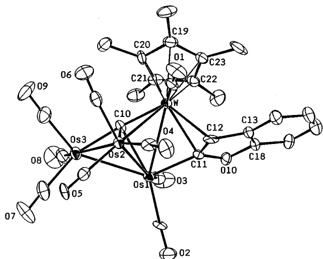
Figure 5. Molecular structure of Cp*WOs 3 (μ 4 -C)(μ-H) 2 (μ-C 8 H 6 O)(CO) 9 ( 10 ), showing the atomic labeling scheme and the thermal ellipsoids at the 30% probability level.
