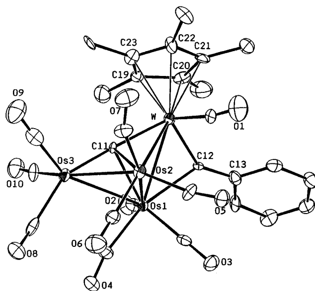
Figure 1. Molecular structure of Cp*WOS 3 ( \mu -C)( \mu -CPh)-(CO) 10 (5), showing the atomic labeling scheme and the thermal ellipsoids at the 30% probability level.
