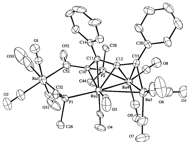
Figure 3. ORTEP plot of compound 4 . Only the ipso carbons of the phenylphosphido groups are shown for clarity. Selected bond lengths (Å) not given in the text: Ru(1)–P(1), 2.437(3); Ru(2)–P(1), 2.406(2); Ru(2)–Ru(3), 3.037(1); Ru(2)–Ru(4), 2.8352(9); Ru(3)–Ru(4), 2.669(1); P(2)–C(10), 1.824(8); Ru(4)–P(2), 2.307(3); Ru(2)–C(10), 2.233(8); C(10)–C(11), 1.46(1); C(11)–C(12), 1.42(1); C(12)–C(13), 1.36(1); Ru(2)–C(11), 2.191(8); Ru(2)–C(12), 2.151(8); Ru(3)–C(13), 2.083(9); Ru(4)–C(13), 2.293(9); Ru(4)–C(12), 2.096(8).
