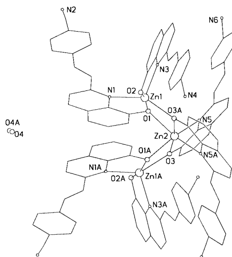
Figure 1. The molecular structure of 1 with labeling scheme. Hydrogen atoms are omitted for clarity. Selected bond lengths (Å) and angles(°): Zn1-O1 2.014(2), Zn1-O2 1.980(3), Zn1-O3A 2.160(3), Zn2-O1 2.205(3), Zn2-O3 2.033(2), Zn1-N1 2.222(3), Zn1-N3 2.120(3), Zn2-N5 2.223(3); O2-Zn1-O1 165.53(12), O2-Zn1-N3 82.79(13), O1-Zn1-N3 111.06(12), O2-Zn1-O3A 97.49(11), O1-Zn-O3A 75.44(9), O1-Zn1-N1 79.50(11), N2-Zn1-N1 108.82(12), Zn1-O1-Zn2 104.05(11), Zn1A-O3-Zn2, O1-Zn2-O3A 74.08(9), O3-Zn2-N5 79.05(11), O1-Zn2-O1A 85.88(13),
