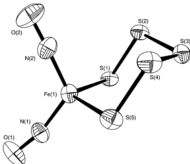
Figure 2. ORTEP drawing and labeling scheme of the [\text{S}_5\text{Fe}(\text{NO})_2]^- anion with thermal ellipsoids drawn at 50% probability.
