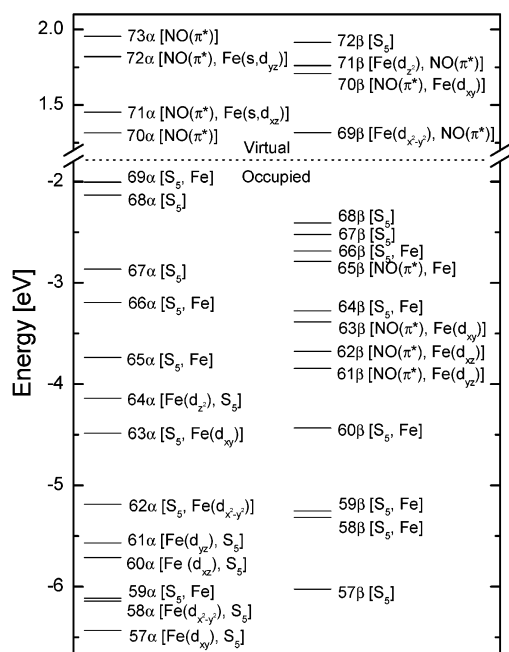
Figure 9. U-B3LYP molecular orbital energy-level diagrams of [S_5Fe(NO)_2]^- . The major compositions of MOs are as indicated. The MOs are divided into spin-up ( \alpha ) levels (left) and spin-down ( \beta ) levels (right). The Fermi level is indicated by a dashed line, below which the orbitals are fully occupied and above which lie the unoccupied virtual MOs.
