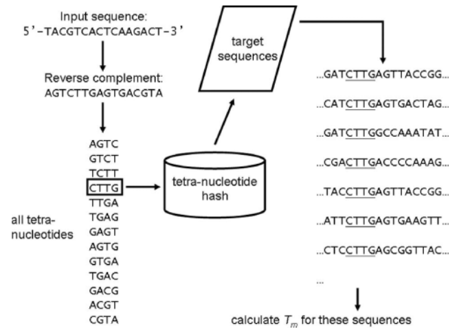
Fig. 2. TNN-hash for fast filtering on primer/probe candidates.
