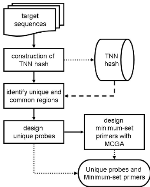
Fig. 1. Overall flow of our integrated primer/probe design algorithm.
