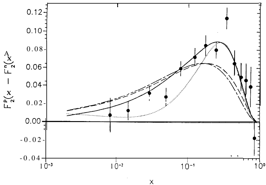
FIG. 4. The structure function difference F_2^p(x) - F_2^n(x) shown as a function of x . The four curves are our predictions using four different input valence distributions for the nucleon - in dash-dotted curve from the distribution extracted from the neutral-current neutrino data, 33 in dashed curve from the charge-current neutrino data, 33 in dotted curve from the input distribution of Harriman et al. , 31 and in solid curve from the distributions of Eichten et al. 30
