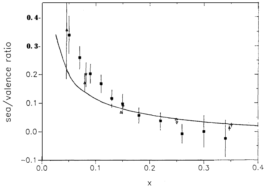
FIG. 3. The ratio 1/2\{\bar{u}(x) + \bar{d}(x)\} / \{u_V(x) + d_V(x)\} as a function of x for Q^2 = 16.85 \text{ GeV}^2 , shown as a function of x . The CDHS data 26 are shown in triangles and the Fermilab E615 data in solid squares. 27
