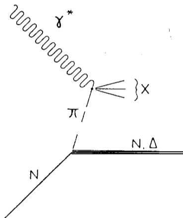
FIG. 1. The processes considered originally by Sullivan. 34
