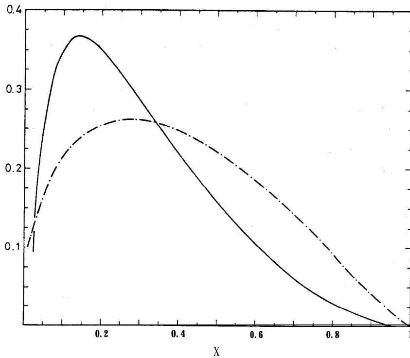
FIG. 6. The valence momentum distributions in the pion. Using our routine to evolve the valence distributions via Altarelli-Parisi equations from Q^2 = 3 \text{ GeV}^2 to Q^2 = 25 \text{ GeV}^2 , the result is displayed as a solid curve. For comparison, the valence momentum distribution (at Q^2 \approx 2.5 \text{ GeV}^2 ) obtained by the NA3 Collaboration 20 in fitting to their Drell-Yan data using \pi^\pm beams is shown as a dash-dotted curve.
