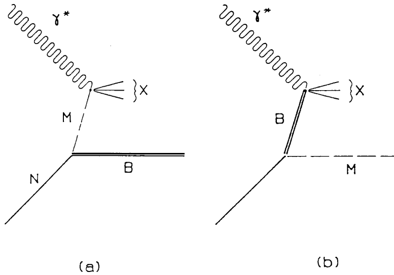
FIG. 2. The generalized Sullivan processes: (a) the virtual photon strikes the cloud meson, and (b) the virtual photon strikes the recoiling baryons. Both scale in the Bjorken limit. The meson and baryon pair (M, B) includes (\pi, N), (\rho, N), (\omega, N), (\sigma, N), (K, \Lambda), (K, \Sigma), (K^*, \Lambda), (K^*, \Sigma), (\pi, \Delta), and (\rho, \Delta) .
