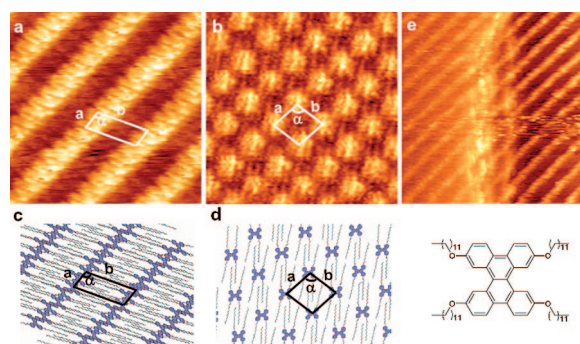
Figure 1. Adlattice structures of 3,6,11,14-tetradodecyloxydibenzo[ g,p ]chrysene for films (a) being subjected to the shear treatment sketched in Figure 2 and (b) prepared by drop cast. (c and d) Proposed adlattices. (e) Face-to-face molecular packing extending across local defects. |\bar{a}| , |\bar{b}| , and \alpha for images a and b are, respectively, 1.04 \pm 0.09 nm, 3.06 \pm 0.13 nm, 115^\circ \pm 3^\circ , and 1.70 \pm 0.11 nm, 1.92 \pm 0.12 nm, 95^\circ \pm 4^\circ . Note that in panels a and c there are two molecules per unit cell because the molecules are zigzagged along \bar{a} , parallel to [01 \bar{1} 0] of the underlying HOPG (lattice is not drawn for clarity). DBC was dissolved and imaged in phenyloctane. The E_{\text{bias}} , I_{\text{tunneling}} , and imaging sizes for images a, b, and e, are, respectively, -0.80 V, 60 pA, 12 \times 12 nm 2 , -0.85 V, 36 pA, 12 \times 12 nm 2 , and -0.80 V, 60 pA, 30 \times 30 nm 2 .
