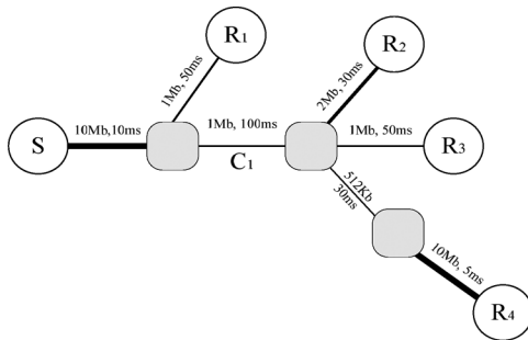
Fig. 6. Simulation topology.
