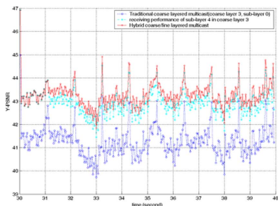
Fig. 8. Y-PSNR of a reconstructed video of Receiver 3 using the hybrid coarse/fine layered multicast compared to a traditional coarse layered multicast scheme. The encoded sequence is the News sequence.
