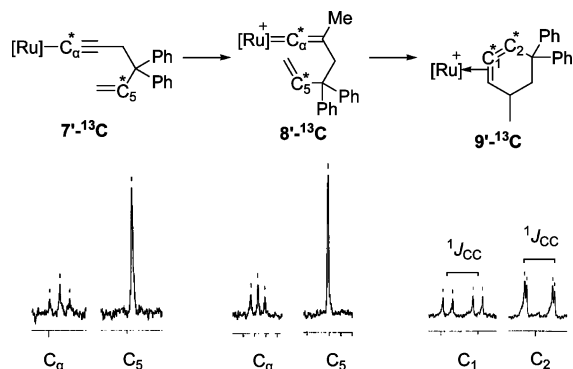
Figure 3. Signal of resonances of enriched ^{13}\text{C} in the ^{13}\text{C} spectra of 7'^{13}\text{C} , 8'^{13}\text{C} , and 9'^{13}\text{C} .
