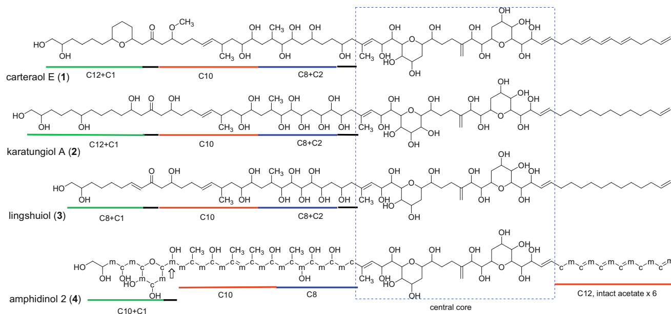
Figure 4. Structures of carteraeol E (1), karatungiol A (2), lingshuiol (3), and amphidinol 2 (4).
