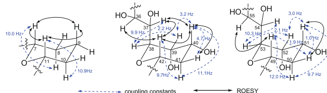
Figure 3. Relative stereochemistries of three tetrahydropyran rings of carteraeol E ( 1 ). Dashed arrows denoted coupling constants and plain arrows denoted ROESY.
