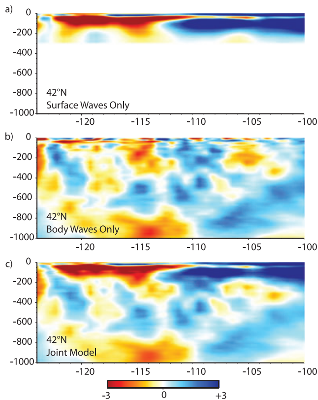
Figure 6. Comparison of the surface-wave only (a), body-wave only (b) and joint model (c) using an E–W vertical cross-section at 42^\circ\text{N} ; (b) emphasizes the poor resolution provided by body-waves at depths smaller than \sim 150 km using the typical station spacing of USArray. In the joint model, the upper 150 km are constrained mainly by the surface-wave data set.
