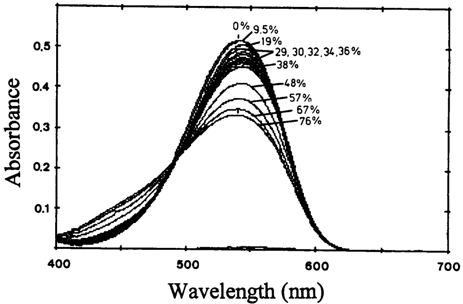
Figure 3 Effect of ethanol concentration (as % v/v) to the absorption spectrum of the pink azo dye. All sample contained 10 \mu\text{M} nitrite and the final acidities were fixed at 34 mM.
