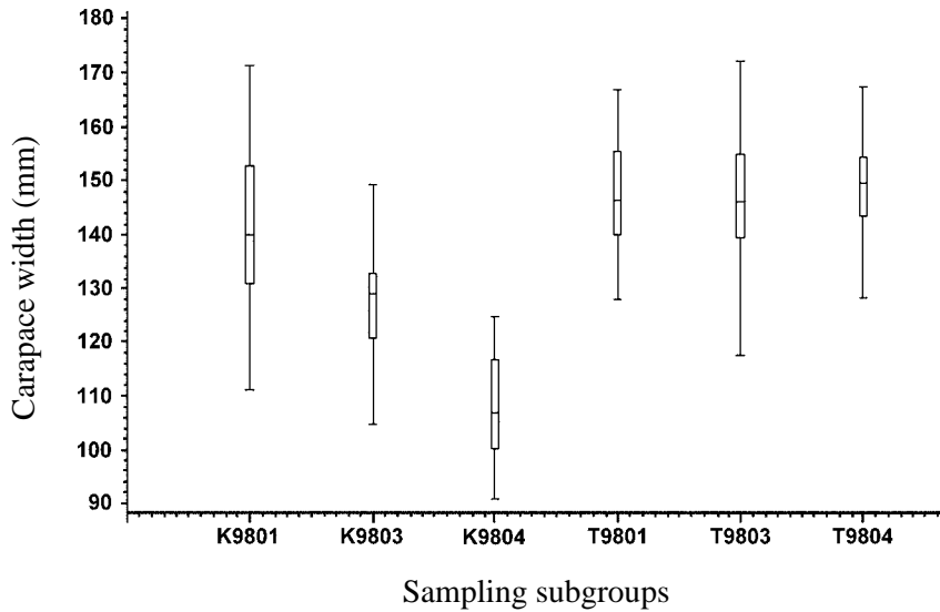
Fig. 3. Box plots for size (carapace width) distribution of Portunus sanguinolentus in each dataset to indicate the mean (horizontal line in rectangular box), the third quartile (Q3, upper boundary of vertical rectangle), the first quartile (Q1, lower boundary of vertical rectangle), and the range (vertical lines).
