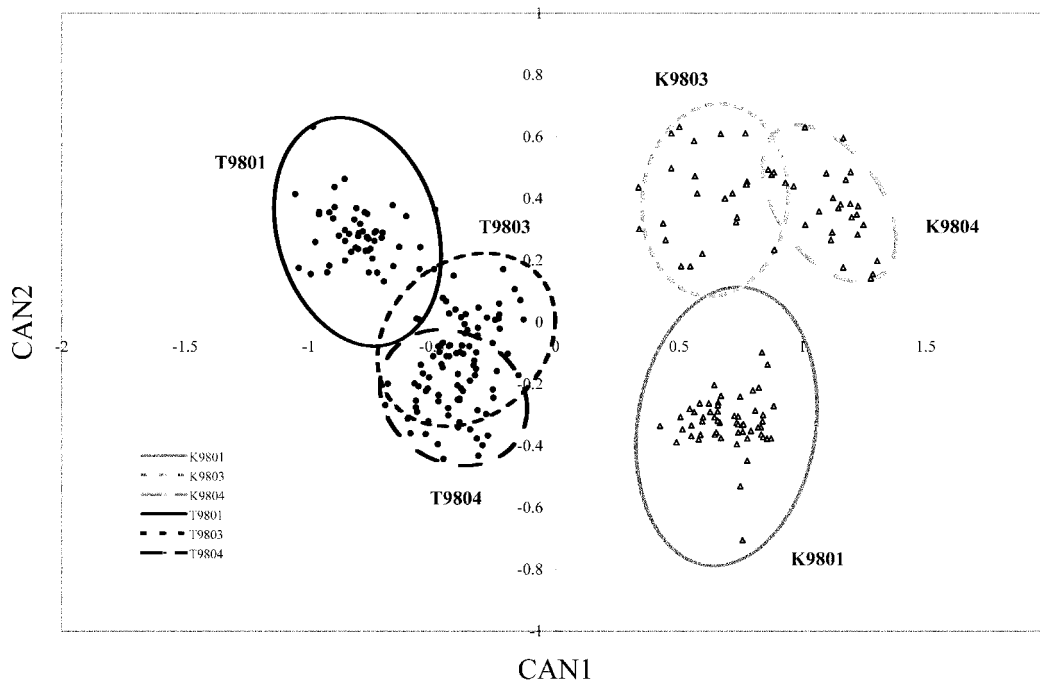
Fig. 5. The canonical variates chart showing the mutual relations of six sampling subgroups based on eight morphometric characters, in which circles represent the 90% ellipsoidal confidence region corresponding to the mean of each subgroup; and where canonical variates are shown with an open triangle and solid circle for data from Keelung Shelf and Taiwan Bank, respectively; and gray circles and black circles represent the 90% ellipsoidal confidence region for Keelung Shelf and Taiwan Bank, respectively.
