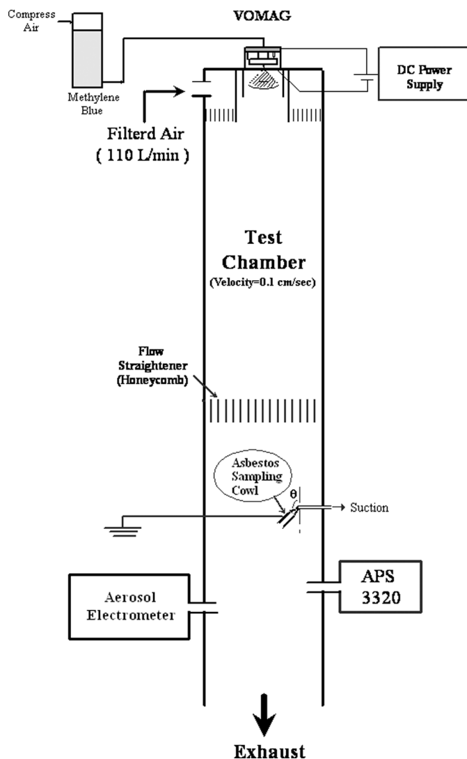
FIG. 1. The schematic diagram of system setup.
