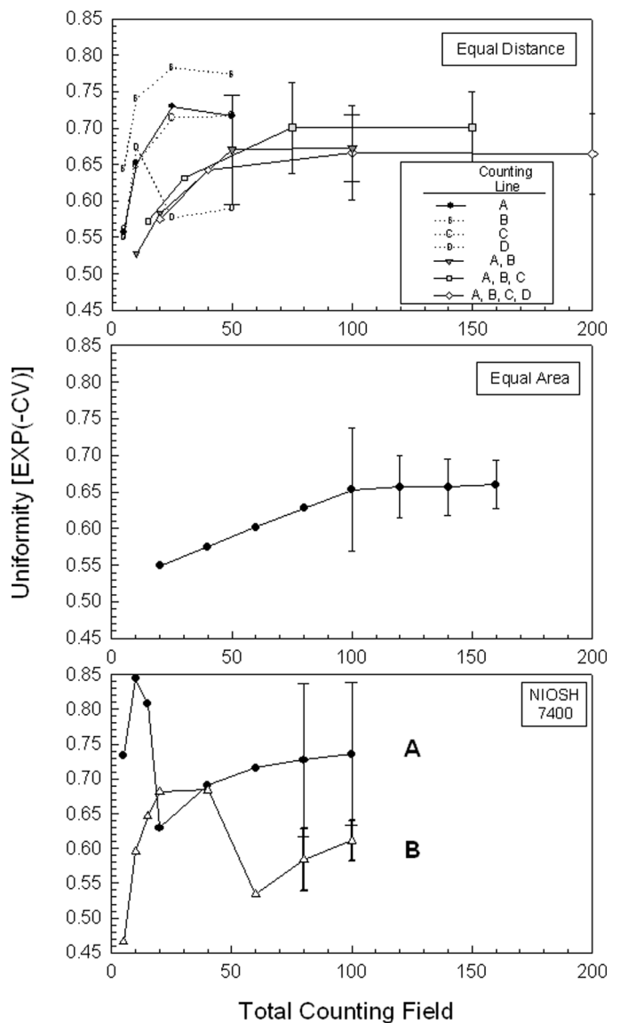
FIG. 9. The uniformity versus total counting fields using (from top) equal distance, equal area, and NIOSH 7400 counting methods.
