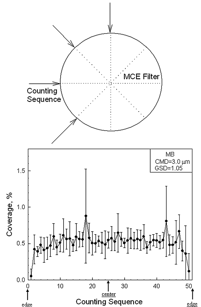
FIG. 5. The particle coverage profile on the MCE filter following equal distance counting method.
