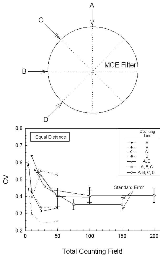
FIG. 6. The CV versus various counting lines and total counting fields using equal distance counting method.
