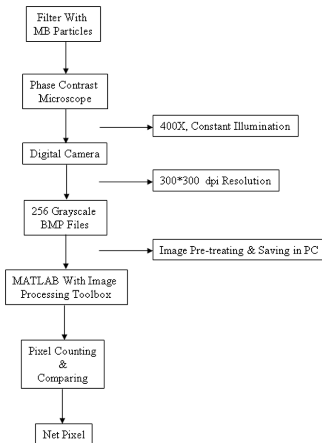
FIG. 2. The flow chart of image processing and particle counting.
