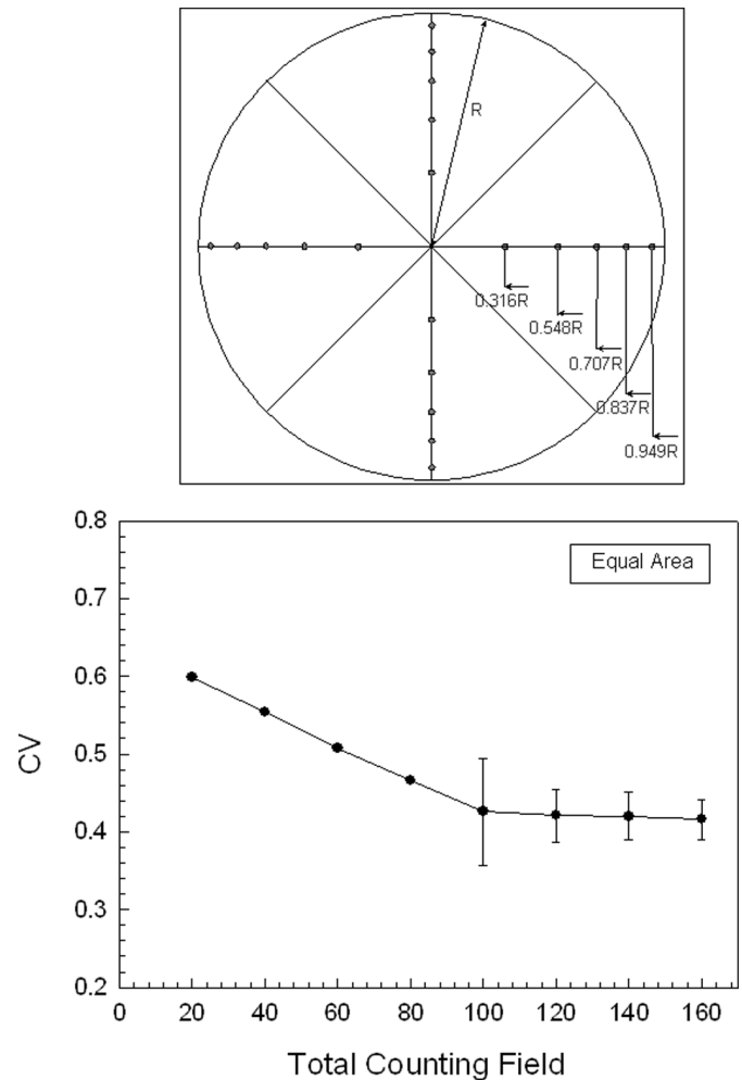
FIG. 7. The CV as a function of total counting fields using equal area counting method.
