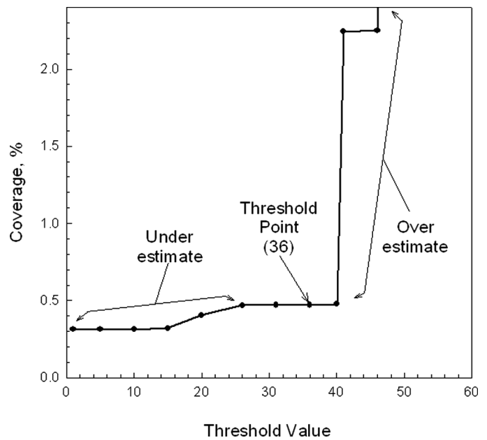
FIG. 4. The determination of threshold value.
