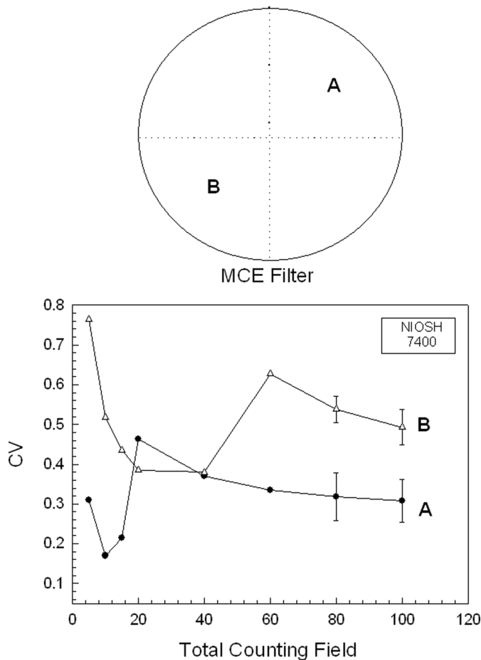
FIG. 8. The CV as a function of total counting fields using NIOSH 7400 counting method.
