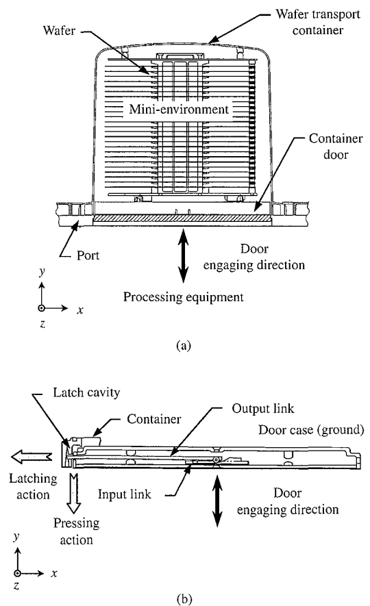
Fig. 1 (a) SMIF environment; (b) Latch mechanism
