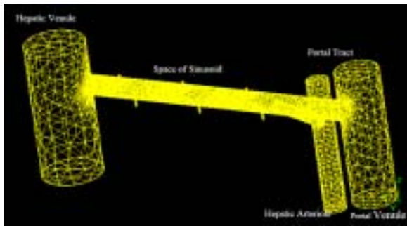
Figure 2. Acinus structure
