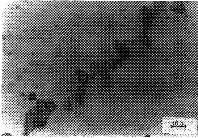
FIG. 2. Grain-boundary precipitates in the Ni-8 at. % Sn sample annealed at 773 K for 1 day.
