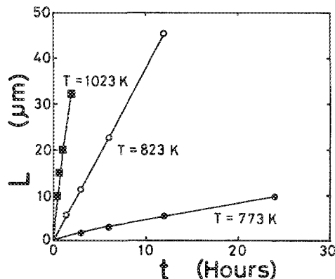
FIG. 3. Averaged size of the cells of the grain-boundary precipitates as a function of annealing time at temperatures of 773 K ( \bullet ), 823 K ( \circ ), and 1023 K ( \blacksquare ).
