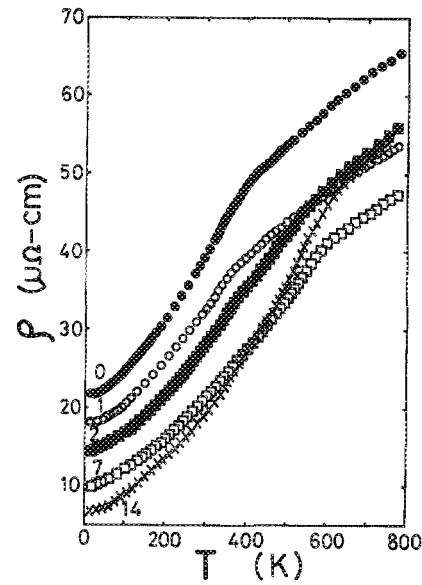
FIG. 4. Electrical resistivity as a function of temperature between 10 and 800 K for Ni-8 at. % Sn samples homogenized at 1325 K ( \bullet ), and annealed at 773 K for 1 day ( \circ ), 2 days ( \blacksquare ), 7 days ( \square ), and 14 days ( \times ).
