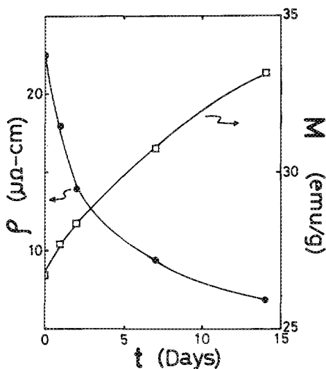
FIG. 6. Electrical resistivity ( \bullet ) at T = 10 K and the magnetization ( \square ) at H = 5 kG and T = 10 K as functions of annealing time for Ni-8 at. % Sn samples annealed at 773 K.
