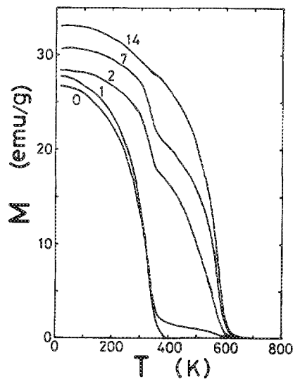
FIG. 5. Magnetization at H = 5 \text{ kG} as a function of temperature between 10 K and 800 K for Ni-8 at. % Sn samples homogenized at 1325 K (No.0), and annealed at 773 K for 1 day (No.1), 2 days (No.2), 7 days (No.7), and 14 days (No.14).
