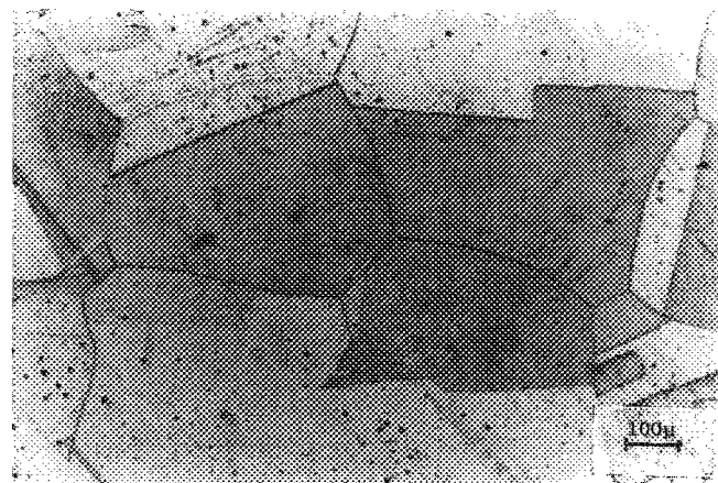
FIG. 1. Grain boundary of the homogenized Ni-8 at. % Sn sample.
