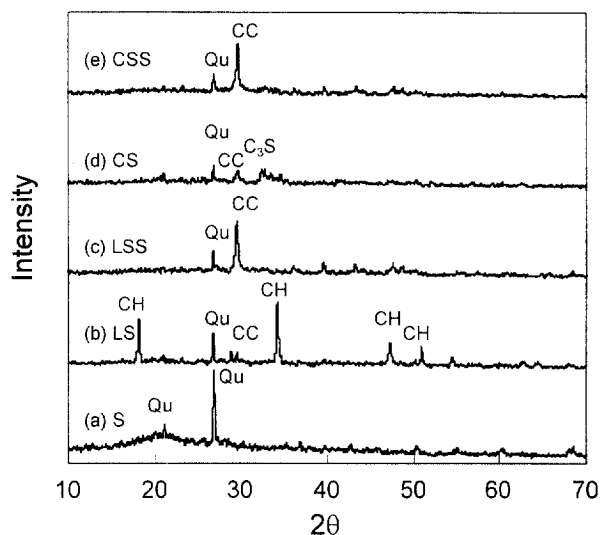
Fig. 1. XRD patterns of: (a) Untreated sewage sludge; (b) Lime-treated sludge; (c) Lime–sodium silicate-treated sludge; (d) Cement-treated sludge; (e) Cement–sodium silicate-treated sludge. *C 3 S: tricalcium silicate (3CaO·SiO 2 ); CH: calcium hydrate; CC: calcium carbonate; Qu: quartz (SiO 2 ); S: untreated sludge; LS: lime-treated sludge; LSS: lime–sodium silicate-treated sludge; CS: cement-treated sludge; CSS: cement–sodium silicate-treated sludge.
