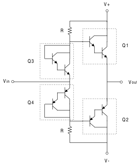
Figure 12. Developed double push-pull circuit for voice coil motor.
