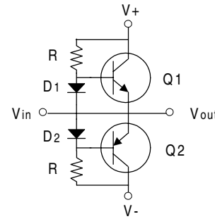
Figure 11. Bias-voltage compensated push-pull amplifier.
