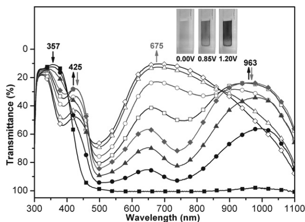
Fig. 4 Electrochromic behavior of polyamide 6b thin film (in CH 3 CN with 0.1 M TBAP as the supporting electrolyte) at 0.00 (■), 0.65 (●), 0.75 (▲), 0.85 (◆), and 0.95 (□) (V vs. Ag/AgCl). 6b + : (solid symbols with black arrows) and 6b 2+ : (hollow symbols with gray arrows).
