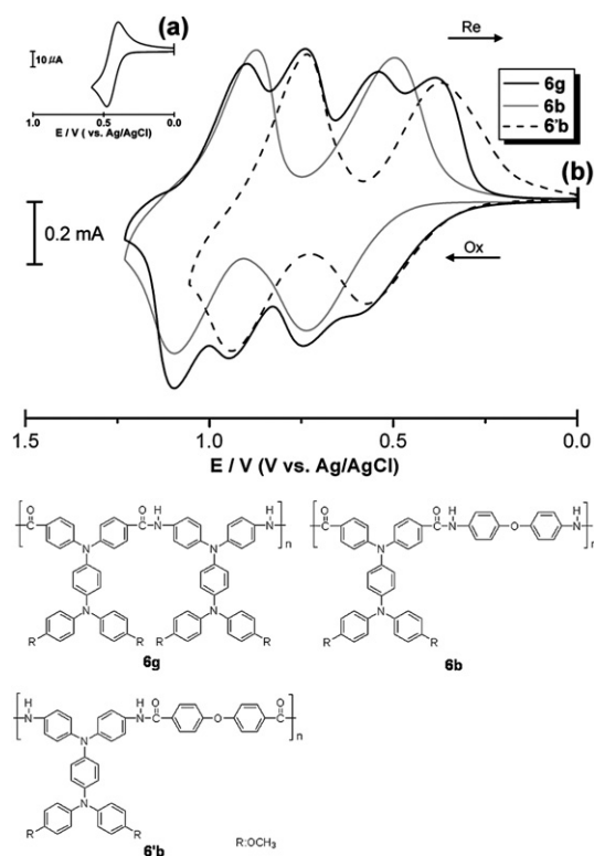
Fig. 1 Cyclic voltammograms of (a) ferrocene (b) polyamides 6g , 6b and 6'b in \text{CH}_3\text{CN} containing 0.1 M TBAP at scan rate = 0.05 V/s.
