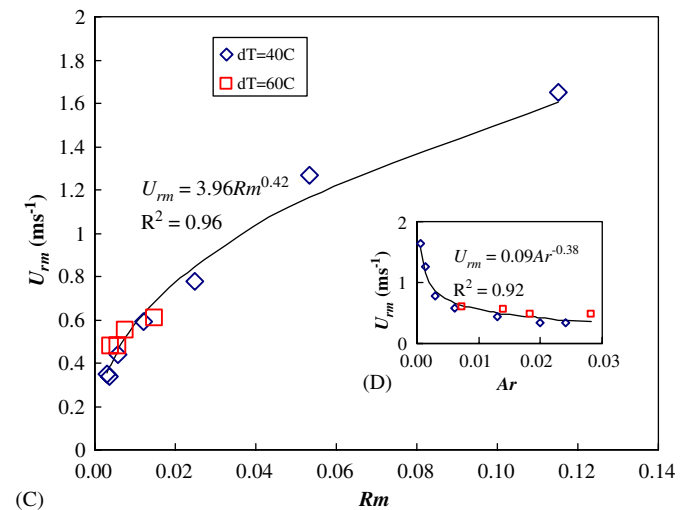
Fig. 9. Maximum floor velocity ( U_{rm} ) fitted with (A) jet momentum ( M ), (B) jet momentum number ( J ), (C) inlet jet momentum ratio ( Rm ), and (D) Archimedes number ( Ar ).
