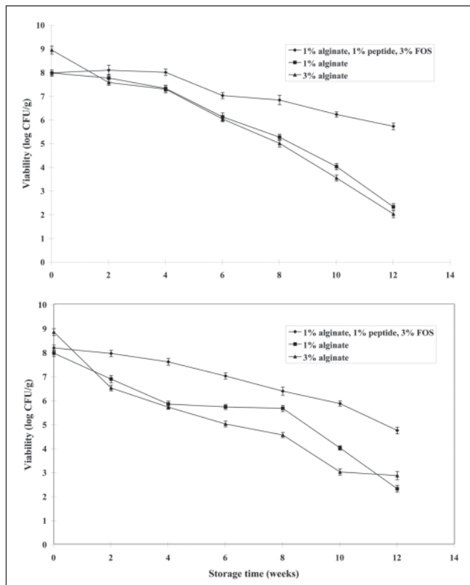
Figure 3—Survival of microencapsulated Lactobacillus and Bifidobacterium in distilled water for 12 wk of storage with 3 different microcapsule formulations.
