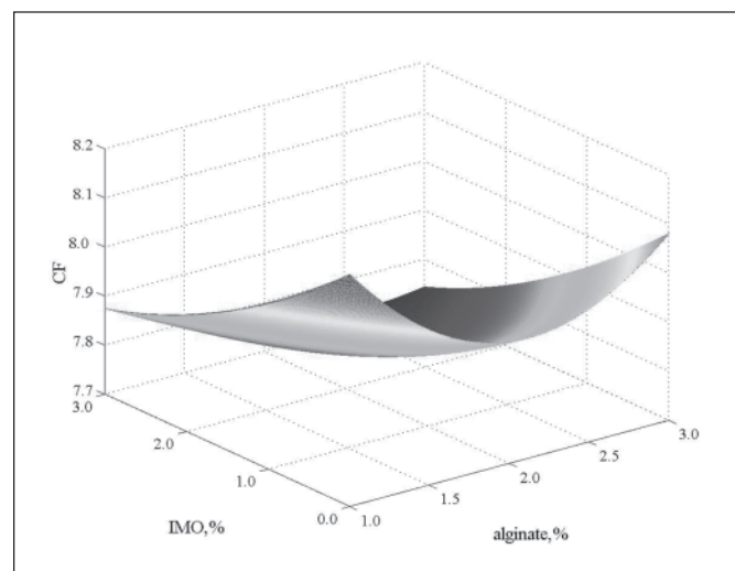
Figure 1—A response surface plot for survivability of probiotic microcapsules showing the effects of sodium alginate and isomaltooligosaccharides (IMO) for constant levels of peptides and fructooligosaccharides (FOS) (1% and 3%, respectively). CF = Composite Function.
