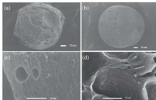
Figure 2—Microstructure of probiotic microcapsules: (a) whole unfractured microcapsules using 1% alginate, 1% peptide, and 3% fructooligosaccharides (FOS) as coating material; (b) whole unfractured microcapsules using 3% alginate as coating material; (c) fractured microcapsules using 1% alginate, 1% peptide, and 3% FOS as coating material; (d) fractured microcapsules using 3% alginate as coating material.
