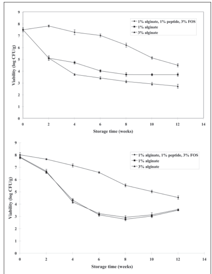
Figure 4—Survival of encapsulated Lactobacillus and Bifidobacterium in distilled water after 12 wk of storage and followed by testing in simulated gastric fluid with 3 different microcapsule formulations.
