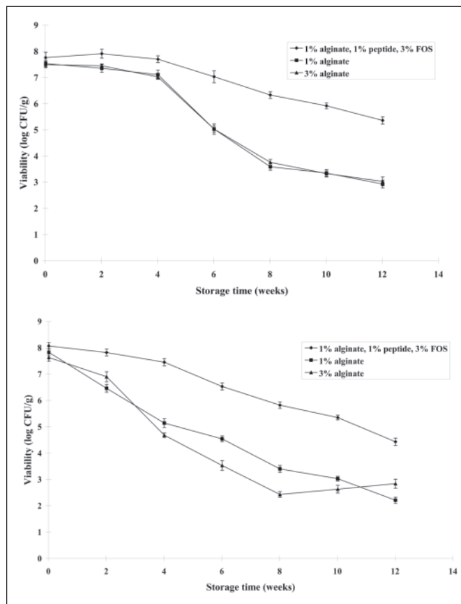
Figure 5—Survival of encapsulated Lactobacillus and Bifidobacterium in distilled water after 12 wk of storage and followed by testing in simulated bile salts with 3 different microcapsule formulations.
