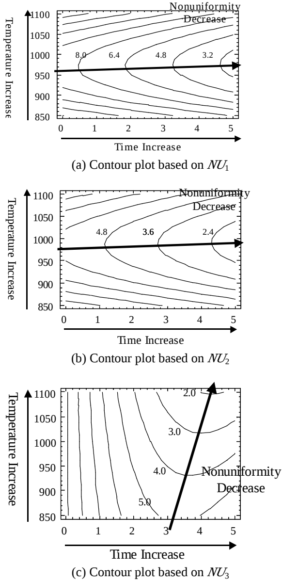
Figure 3: Response surface contour plots
