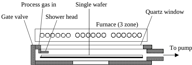
Figure 1: Single-wafer rapid thermal chamber
